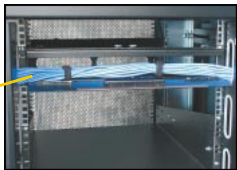
Horizontal Enclosed Wire Management (hinged door)
